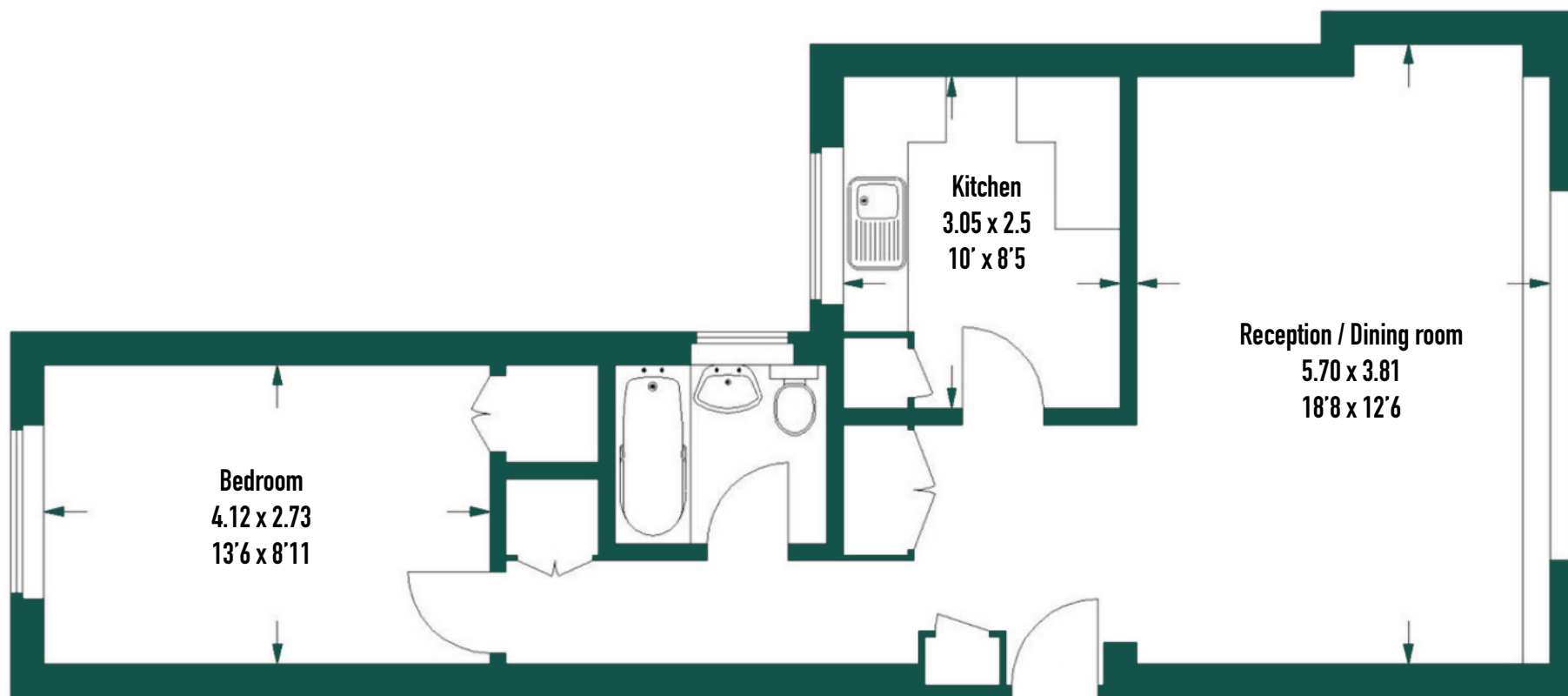
THIRD FLOOR
