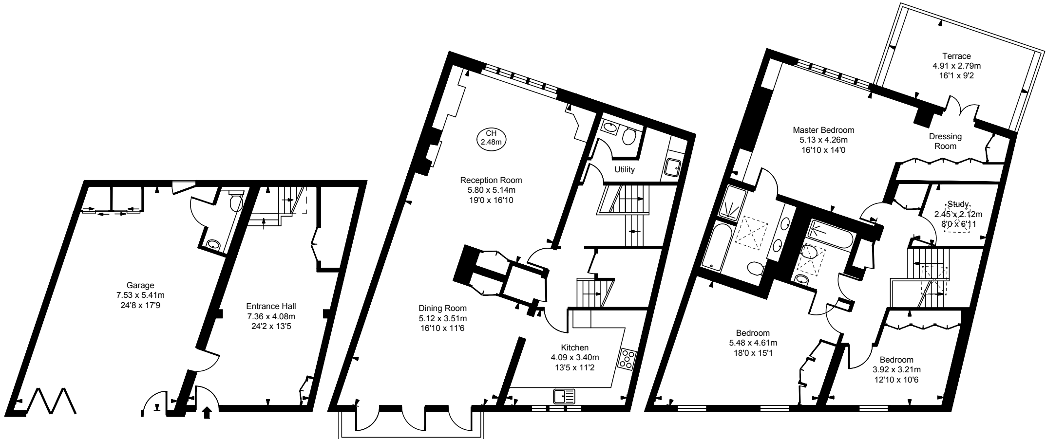
Ground Floor Approximate Gross Internal Area 70.54 sq m / 759 sq ft
